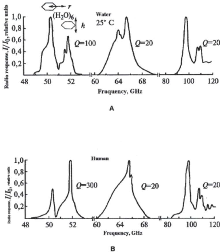
FIGURE 4. Resonant spectra of water (a) and tissues of the organism (b).
